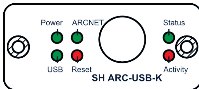
Frontblende SH ARC-USB-K
